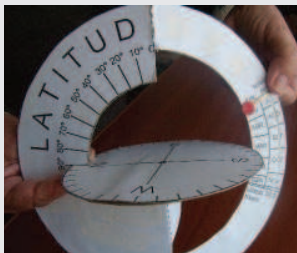
Fig. 22a and 22b: The demonstrator showing the Sun over the horizon for half a year and below the horizon for a half a year.
