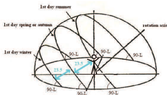
Fig. 10: Three different solar paths (1st day of spring or autumn, 1st day of summer, and 1st day of winter).
