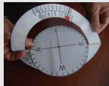
Fig. 23a, 23b and 23c: The Sun rises on the first day of each season: left - 1st day of summer, center - 1st day of spring or autumn, and right - 1st day of winter (in the Northern Hemisphere). On the equator the Sun's path is perpendicular to the horizon. The Sun rises at almost the same point every season. The angular distances between sunrises are only 23.5° (the ecliptic obliquity). In more extreme latitudes the Sun's path is more inclined and the distances between the three sunrise points increase (figures 17 and 19).
