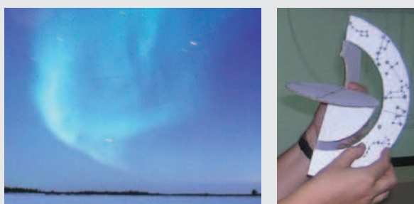
Fig. 9a and 9b: Stars setting in Enontekiö in Lapland (Finland). The angle of the star path relative to the horizon is 90^\circ minus the latitude. Note that the star paths are shorter than in the previous photo because the aurora borealis forces a smaller exposure time (Photo: Irma Hannula).
