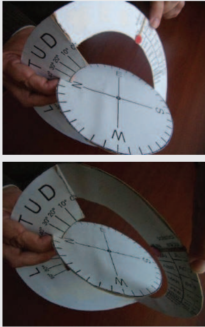
Fig. 11a and 11b: Preparing the solar demonstrator for the Northern Hemisphere at latitude +40^\circ .
