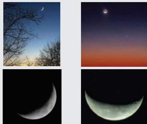
Fig. 28a: Slanting crescent Moon, Fig. 28b: Smiling Moon.
