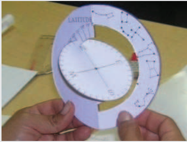
Fig. 2: Using the demonstrator: this is an example of a demonstrator for the Northern Hemisphere using constellations from Table 1.
