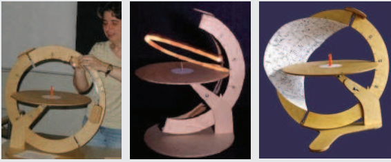
Fig. 25a: XXL wooden demonstrator. Fig. 25b: Stellar wooden demonstrator. Fig. 25c: With a camera it is possible to photograph the solar path using a large exposure time. (Photos: Sakari Ekko).
